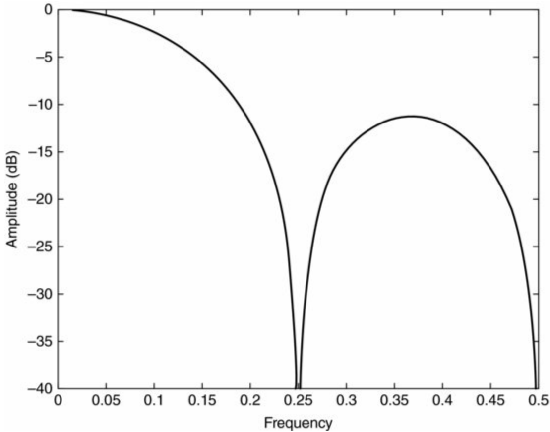
Figure 3.1 Frequency Response of a [1 \ 1 \ 1 \ 1] / 4 Nonrecursive Filter
