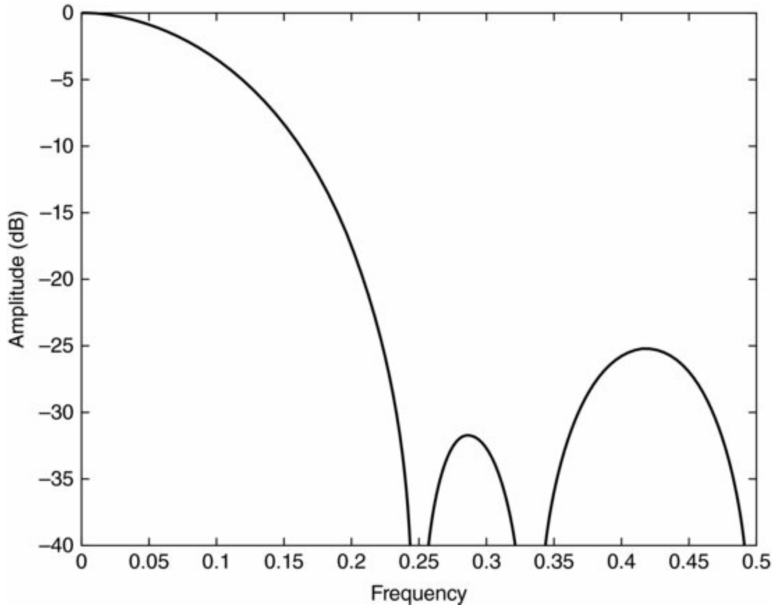
Figure 3.4 Frequency Response of a [1\ 2\ 3\ 3\ 2\ 1] / 12 Nonrecursive Filter
