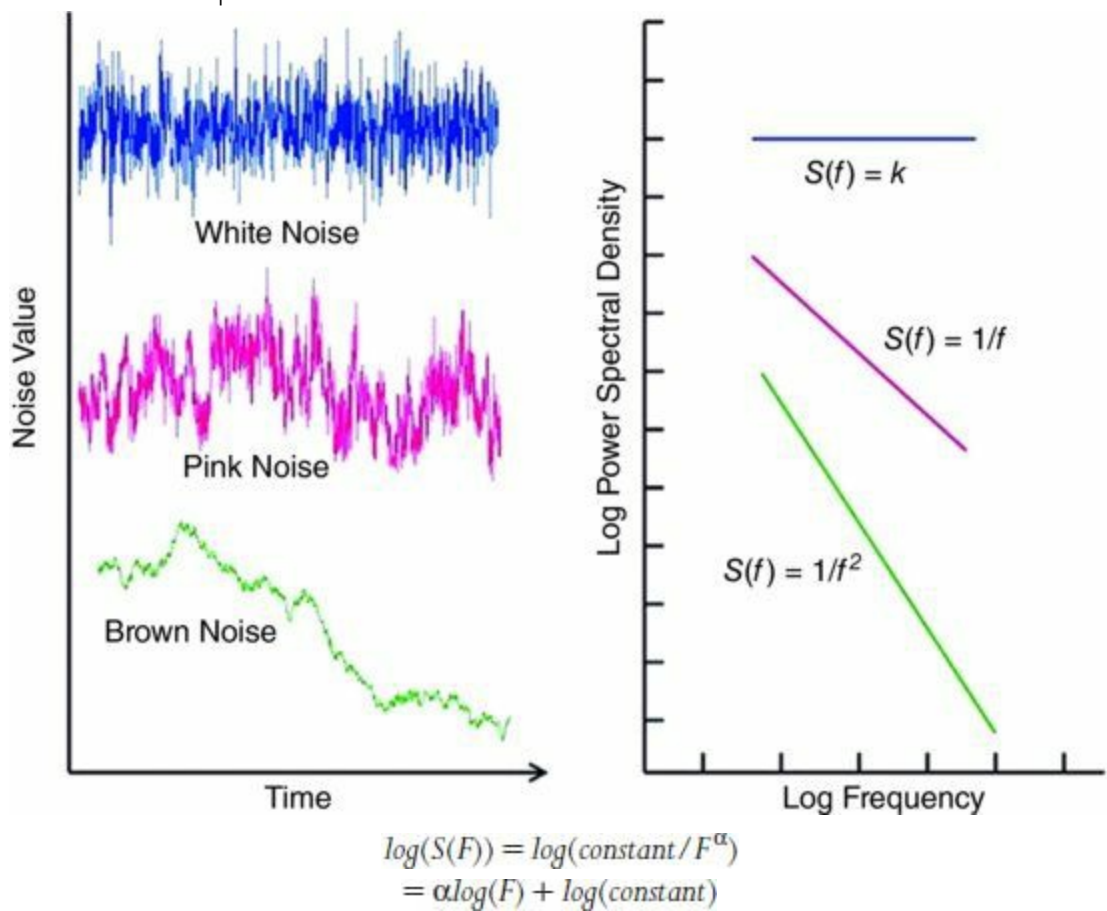
Figure 6.1 Time Series and Spectral Densities for Several Kinds of Noise
