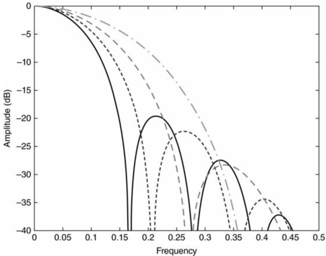
Figure 3.7 Modified Least-Squares Quadratics Filter Frequency Responses
