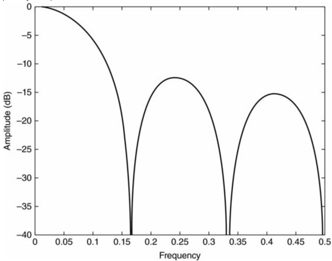
Figure 3.2 Frequency Response of a [1 1 1 1 1 1] / 6 Nonrecursive Filter
