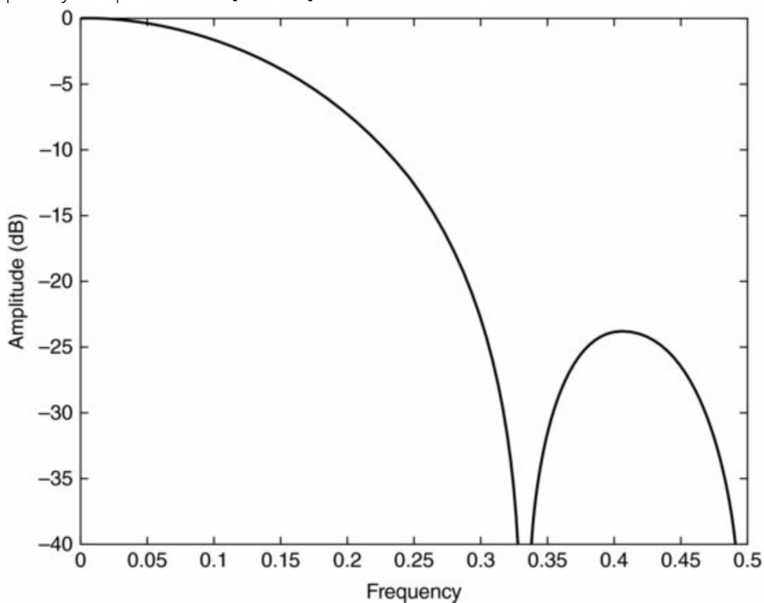
Figure 3.3 Frequency Response of a [1 2 2 1] / 6 Nonrecursive Filter
