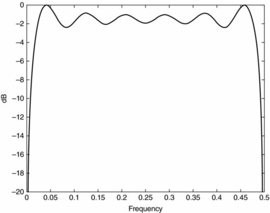
Figure 14.2 Frequency Response of a 23-Element Hilbert Transformer
